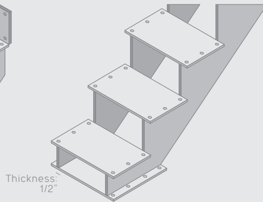
BOTTOM OF THE STAIRS Fixed with a flat plate
