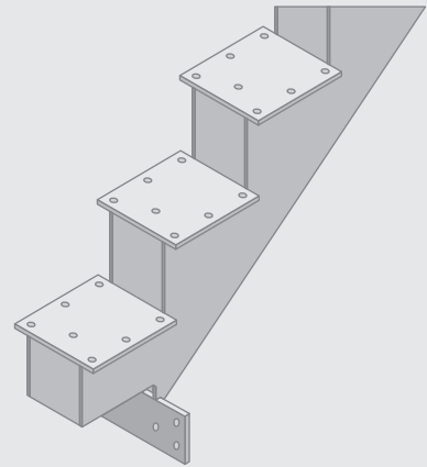
Fixed with an angle mounting plate (finishing plate not available)
