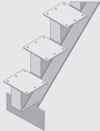
Fixed with an angle mounting plate (finishing plate not available)
