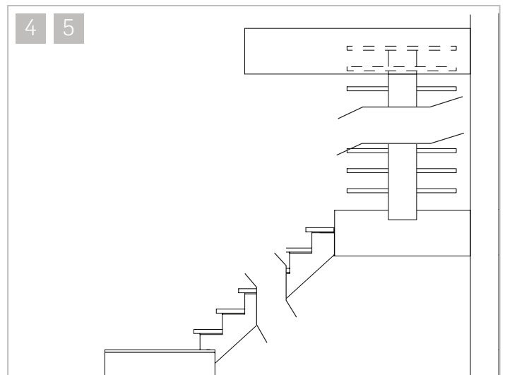
STAIRCASE WITH CHANGE(S) IN DIRECTION
