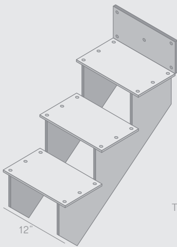
TOP OF THE STAIRS
