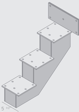
TOP OF THE STAIRS
