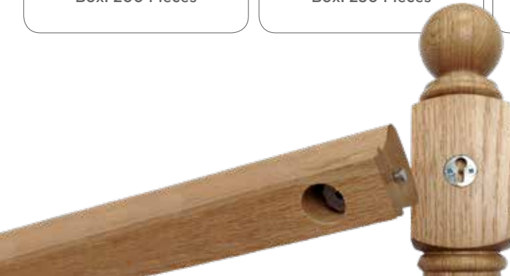
ZIPBOLT UT MICRO FOR SMALL PROFILE RAILS (16.600)
